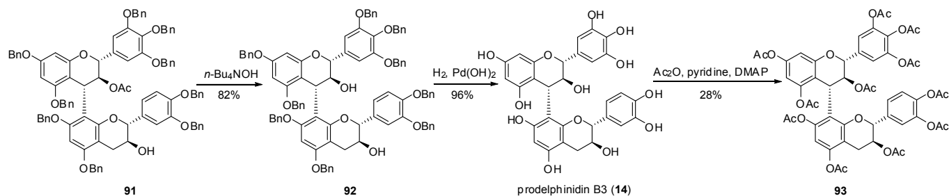
Scheme 20. Synthesis of prodelpinidin B3 ( 14 ) and its peracetate 93
