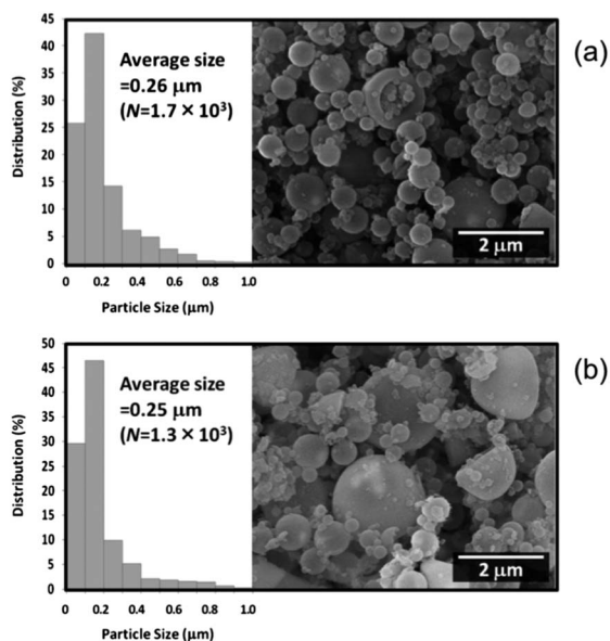
Fig. 2 SEM images of the particles and their particle size distributions (inset). (a) After heating in \text{N}_2 at 973 K. (b) After agitating the sample heat-treated at 973 K in 1 M HCl ( \text{Co@SiO}_2 ).
