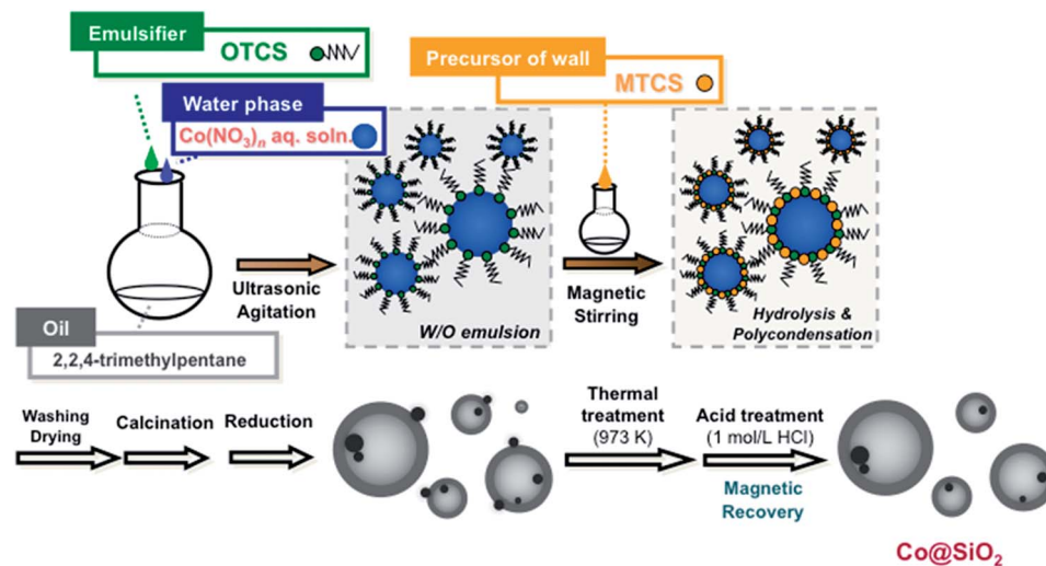
Scheme 1 Schematic drawing of the preparation of Co@SiO 2 particles.
