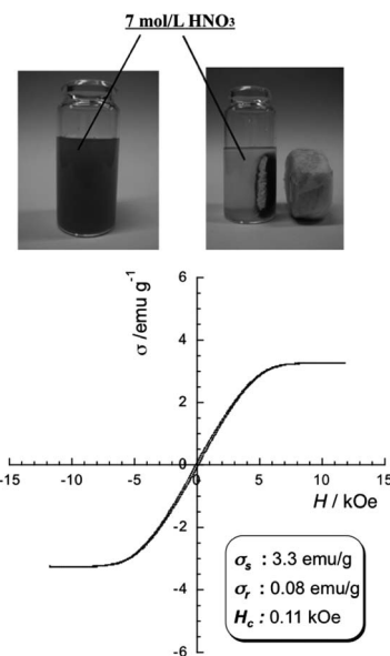
Fig. 7 (Top) Photograph of Co@SiO 2 -SPS particles attracted to a magnet after they were immersed in 7 M HNO 3 to oxidize the thiol group. (Bottom) Magnetization curves of Co@SiO 2 -SPS measured at room temperature.
