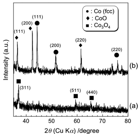
Fig. 1 XRD patterns of (a) the precipitate from the W/O emulsion containing \text{Co}(\text{NO}_3)_2 calcined at 873 K and (b) reduced (a) in \text{H}_2 gas at 773 K.
