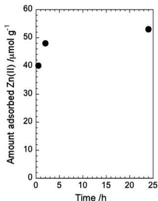
Fig. 8 Time course of adsorption of zinc ions onto Co@SiO 2 -SPS (the initial concentration of 0.4 mM).
