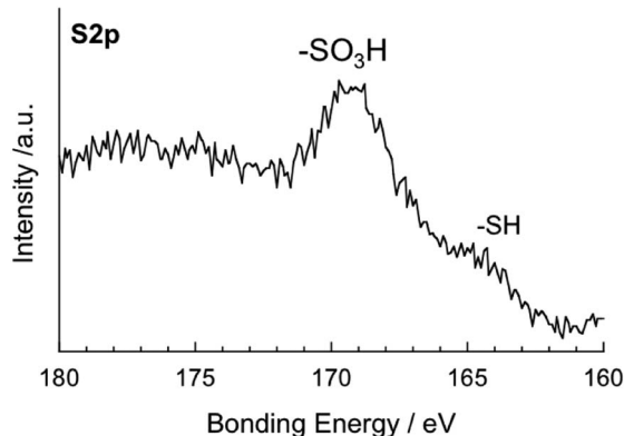
Fig. 5 XPS S2p core-level spectrum of Co@SiO 2 -SPS.
