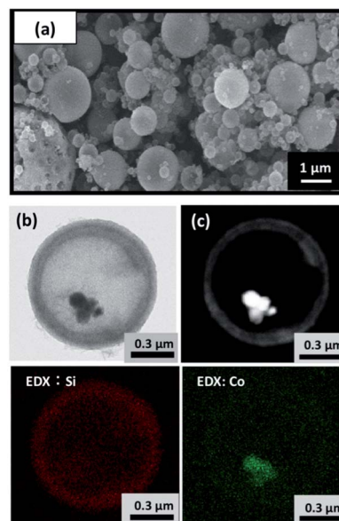
Fig. 6 (a) SEM, (b) TEM, and (c) STEM dark-field images of Co@SiO 2 -SPS. Elemental mapping images of Si and Co are shown at the bottom.
