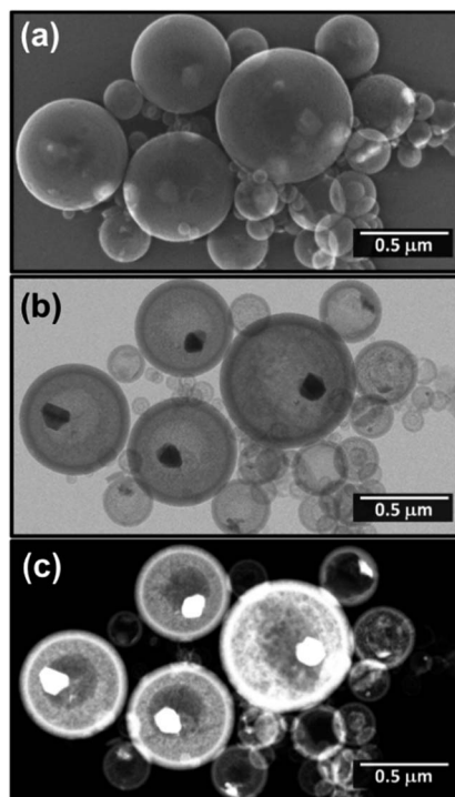
Fig. 3 (a) SEM image, (b) bright-field TEM image, and (c) STEM dark-field image of \text{Co@SiO}_2 .
