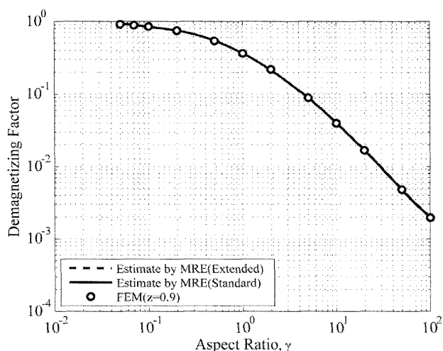
Fig. 5 Three types of demagnetizing factors at the Z position 0.9, which are estimated from Eq. (4) with coefficient equation (5) (extended), from Eq. (4) with coefficient values in Table 1 (standard), and from FEM.
