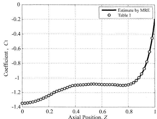
Fig. 4 The results of approximation of the coefficient C_1 in Table 1 from the multiple regression equation (5).
