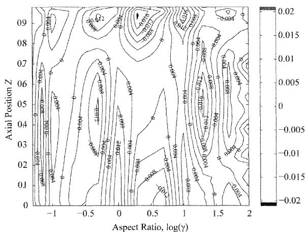
Fig. 6 Error ratio of the demagnetizing factor from Eq. (4) to that from FEM.
