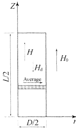
Fig. 1 The computation model for the finite element analysis.
