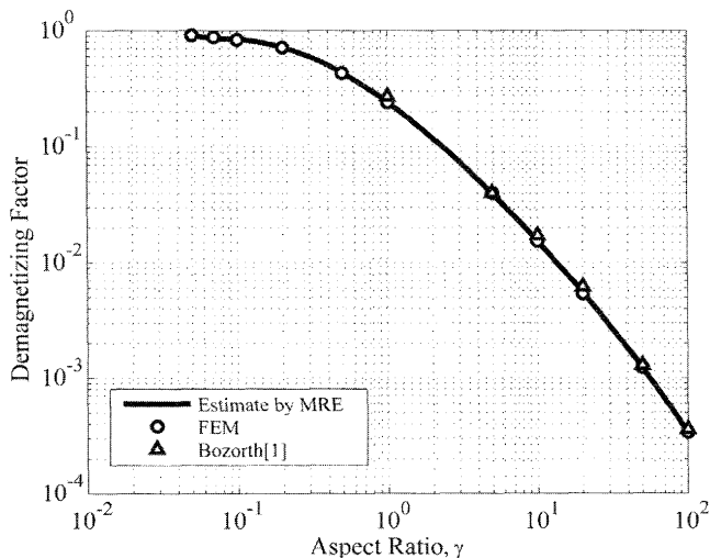
Fig. 2 Comparison of approximated fluxmetric demagnetizing factors at the midplane calculated using FEM, Eq. (3), and data from [1].
