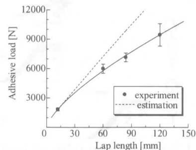
Fig.1 Influence of Lapping Length to Adhesive Load
