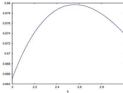
Fig. 3: This is a plot of f(\rho_{\min}) as a function of b = \frac{1}{\sinh \rho_{\min}} . The function f(\rho_{\min}) has a single maximum with maximal value \tau_c ( \sim 0.68 ).
