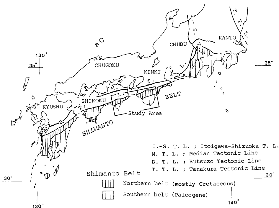
Fig. 1 Index map of the study area.
