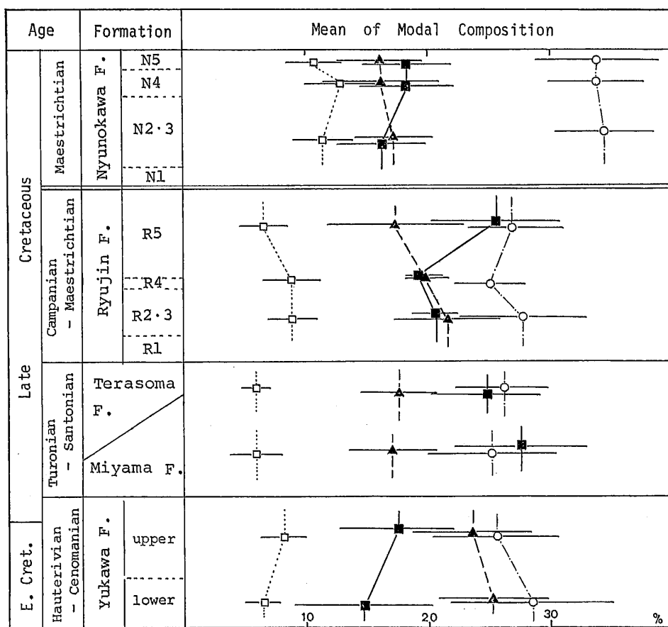
Fig. 16 Stratigraphic change of sandstone composition in the Cretaceous sequences of the Shimanto Supergroup in the Kii Peninsula.
