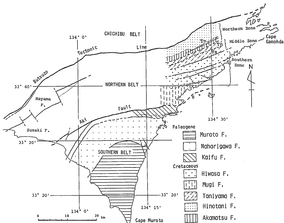
Fig. 2 Generalized geologic map of the Shimanto Belt in eastern Shikoku. Compiled from KUMON (1981), KUMON and INOUCHI (1976) and KARO (1961), and partly modified as mentioned in the text.
