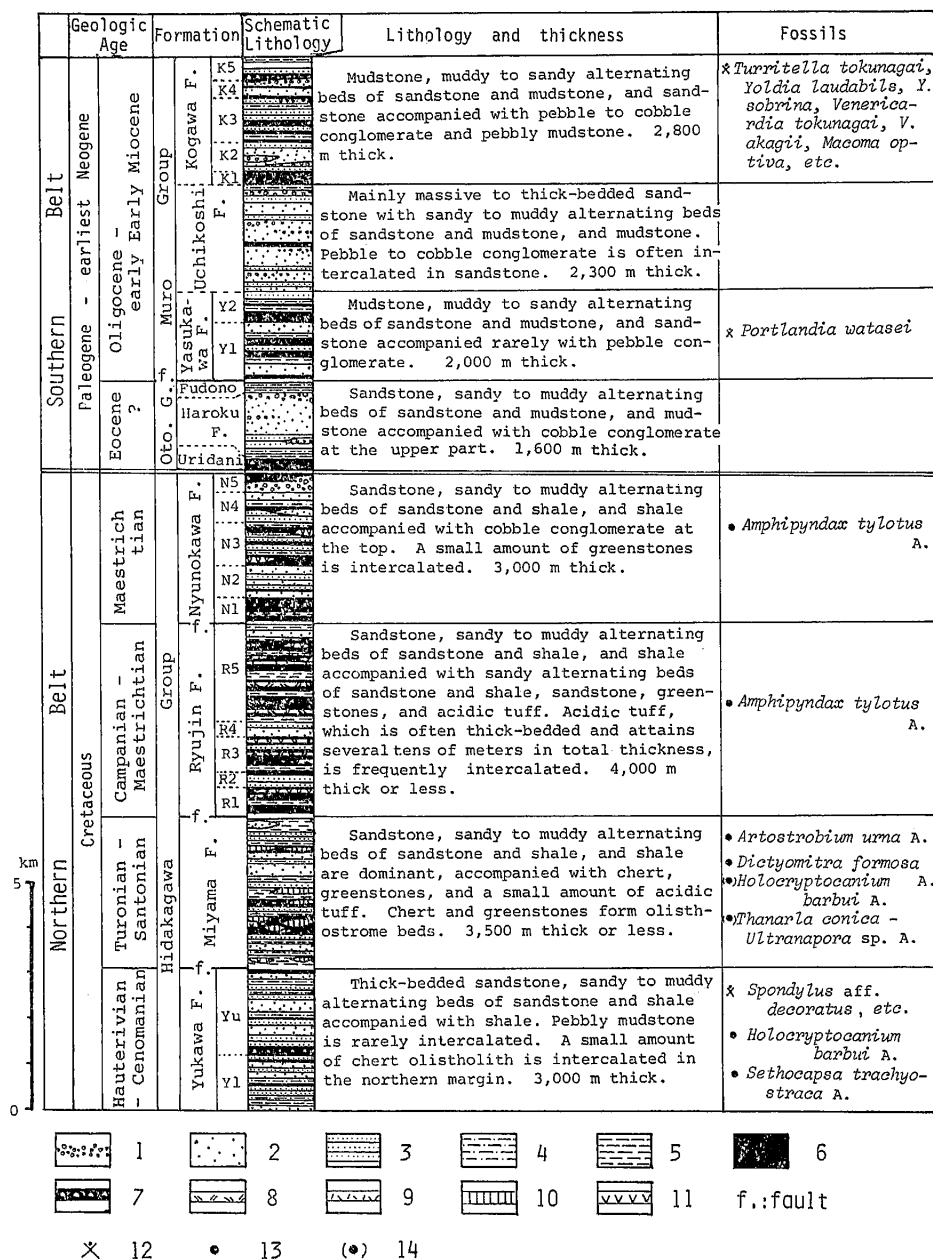
Fig. 5 Stratigraphy and lithology of the Shimanto Supergroup in the central part of the Kii Peninsula. Compiled from K.S.R.G. (1975), Suzuki et al. (1979), Tateishi et al. (1979), Tokuyoka et al. (1981), Kumon and K.S.R.G. (1981) and unpublished data of K.S.R.G.
