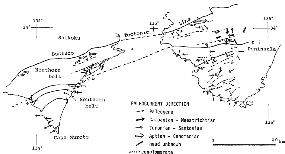
Fig. 13 Diagrammatic sketch of the paleocurrents of the Shimanto Supergroup in eastern Shikoku and Kii Peninsula. Compiled from KUMON (unpub. data), MIYAMOTO (1980), KUMON and INOCHI (1976), KATTO and ARITA (1966) and TAIRA et al. (1980) in eastern Shikoku, and TANAKA (1974), NAKAZAWA et al. (1979), TOKUOKA et al. (1981), and K.S.R.G. (1975, and unpub. data) and TATEISHI (1978).
