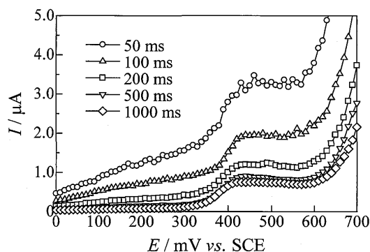
Fig. 4 Effect of the delay time ( \tau_d ) on laser pulse sampled DC voltammogram
