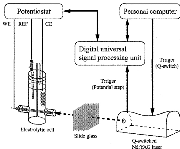
Fig. 2 Schematic diagram of the experimental setup for laser pulse sampled DC voltammetry
