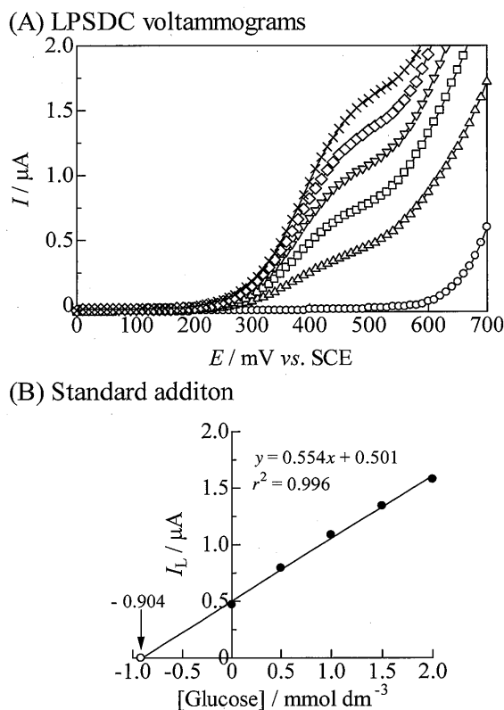
Fig. 5 Laser pulse sampled DC voltammograms of glucose in bovine serum and the relationship between the added quantity of glucose and the limiting current. \tau_d : 1000 ms; time constant: 20 ms; laser pulse intensity: ca. 90 mJ/pulse; supporting electrolyte: 0.1 mol \text{dm}^{-3} NaOH. (A) Laser pulse sampled DC (LPSDC) voltammograms: \circ , the blank solution (45 \text{cm}^3 of 0.1 mol \text{dm}^{-3} NaOH); \triangle : the blank solution + bovine serum 5 \text{cm}^3 ; \square : 0.5 mmol \text{dm}^{-3} glucose added; \nabla : 1.0 mmol \text{dm}^{-3} added; \diamond : 1.5 mmol \text{dm}^{-3} added; +, 2.0 mmol \text{dm}^{-3} added. (B) the relationship between the added quantity of glucose and the limiting current in the standard addition method.
