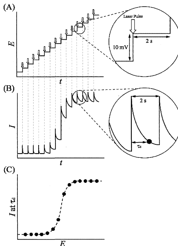
Fig. 1 Principle of laser pulse sampled DC voltammetry (A) potential step and laser pulse irradiation, (B) current at each potential step and laser pulse irradiation, and (C) laser pulse sampled DC voltammogram
