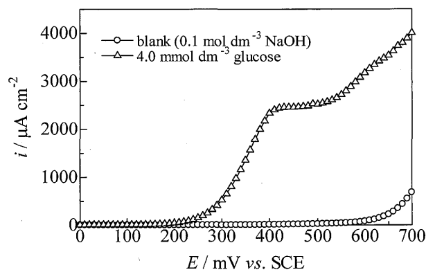
Fig. 3 Laser pulse sampled DC voltammograms for electrooxidation of glucose at the Cu electrode
