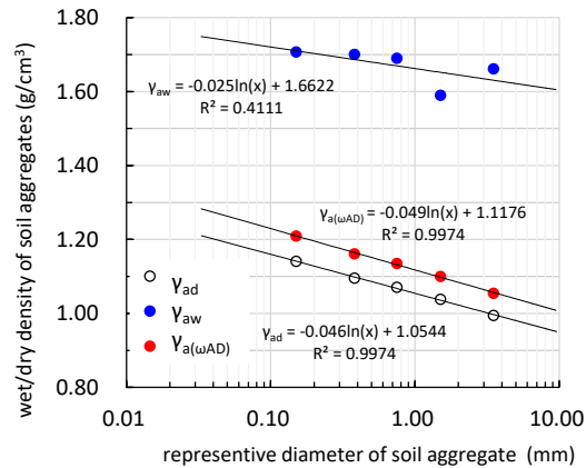
図 I-2. 飽和, 風乾および絶乾土粒密度 Soil aggregate density with soil water
