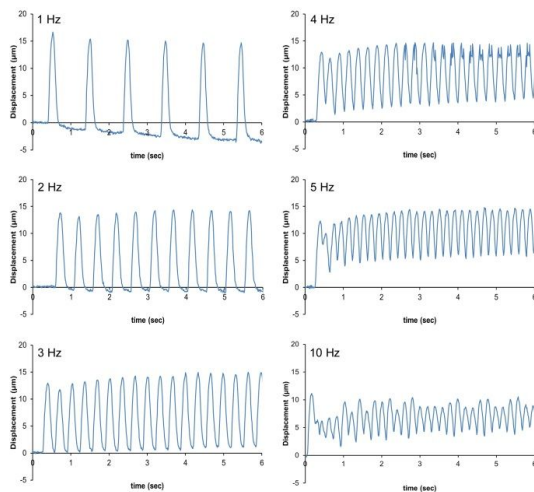
Fig. 6 Response of the micro pillar actuator to electrical pulse stimulation at each frequency.
