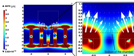
Fig. 2 Magnetic force distribution on the cross section in Fig. 1(a).
