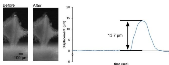
Fig. 7 Response of micro pillar actuator to single electric pulse stimulation at 2 Hz frequency.
