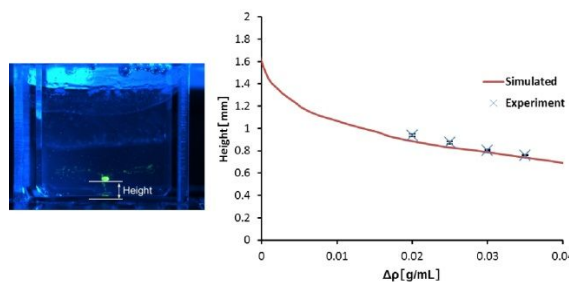
Fig. 3 Relationship between solution density and particle density difference and assembly height. Error bars mean SD.
