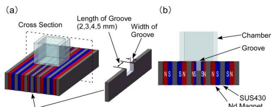
Fig. 1 (a) Schematic illustration of the experimental setup with the grooved SUS430 plate. (b) Cross sectional view of the experimental setup.
